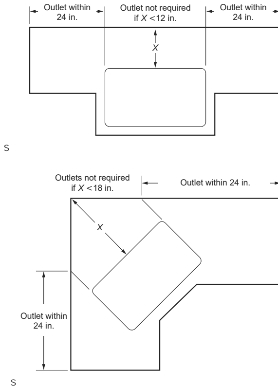
FIGURE E3901.4.1 DETERMINATION OF AREA BEHIND SINK OR RANGE
